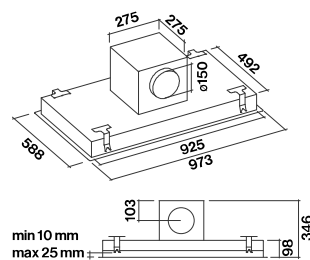
Motor SLIM
