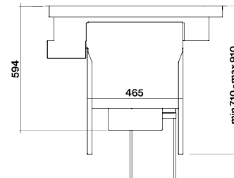
Vista frontal
